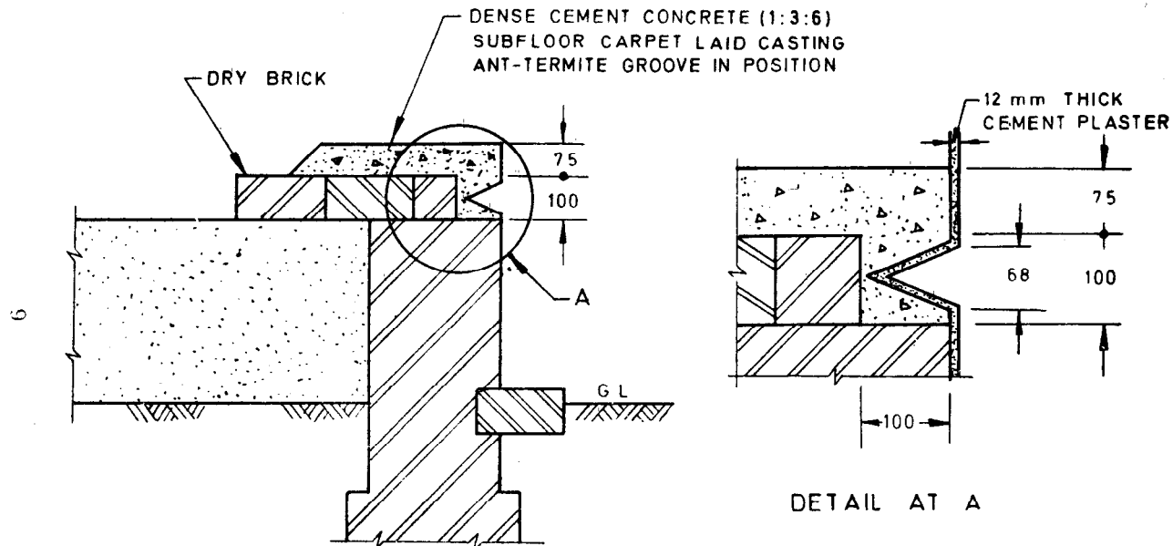
FIG. 3 ANTI-TERMITE CONSTRUCTION — STAGE 3
