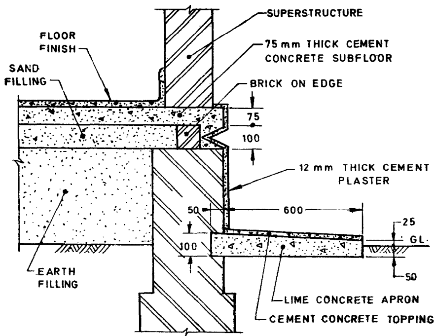
FIG. 9 ANTI-TERMITE CONSTRUCTION — FINAL RECOMMENDATIONS
