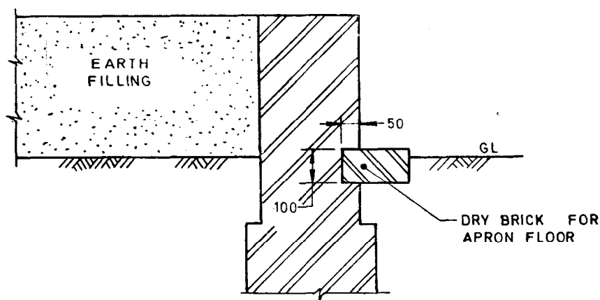
FIG. 1 ANTI-TERMITE CONSTRUCTION — STAGE 1
