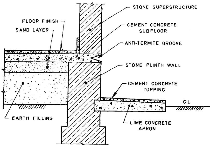
FIG. 10 ANTI-TERMITE CONSTRUCTION IN STONE MASONRY WALL
