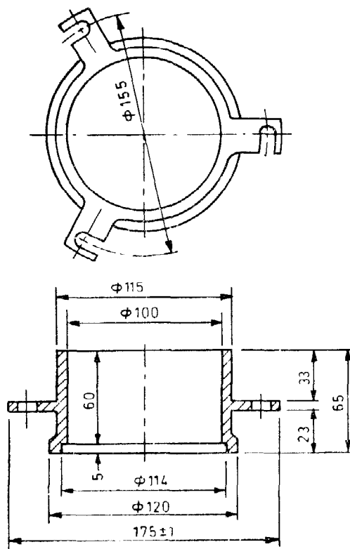
FIG. 7 EXTENSION COLLAR
