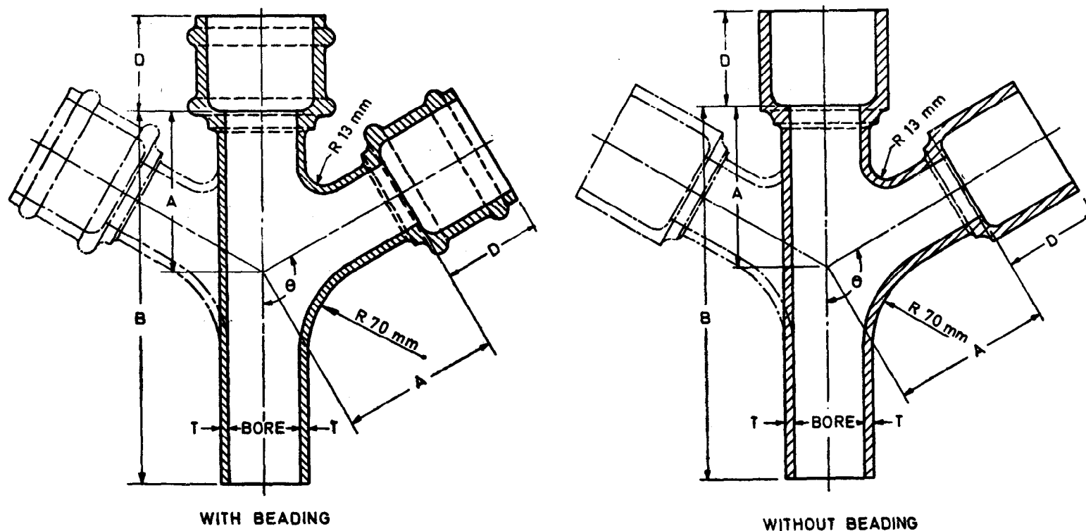
FIG. 6 SINGLE AND DOUBLE EQUAL JUNCTIONS
