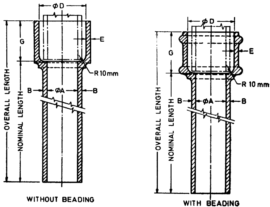
FIG. 1 SINGLE SOCKETED PIPE
