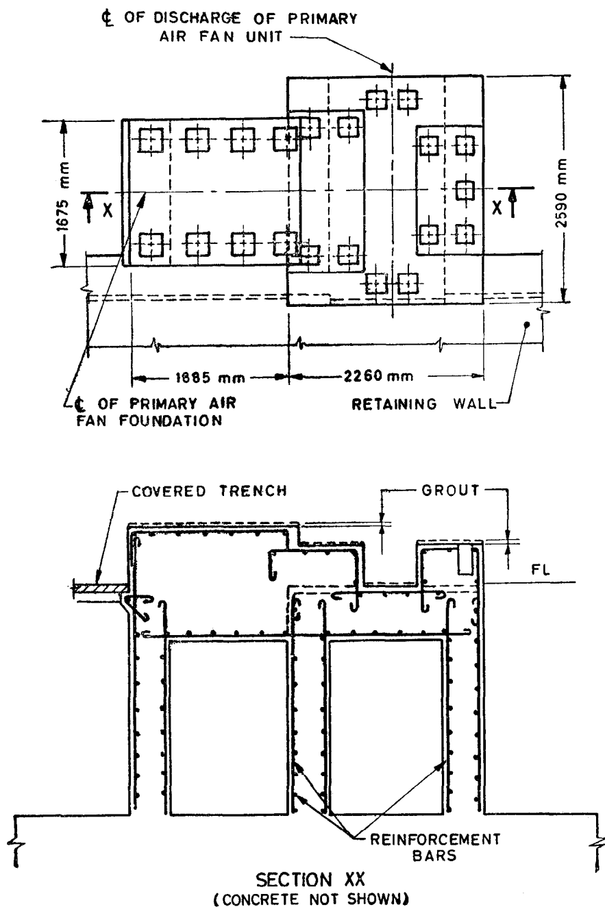
FIG. 2 TYPICAL FOUNDATION FOR PRIMARY AIR FAN
