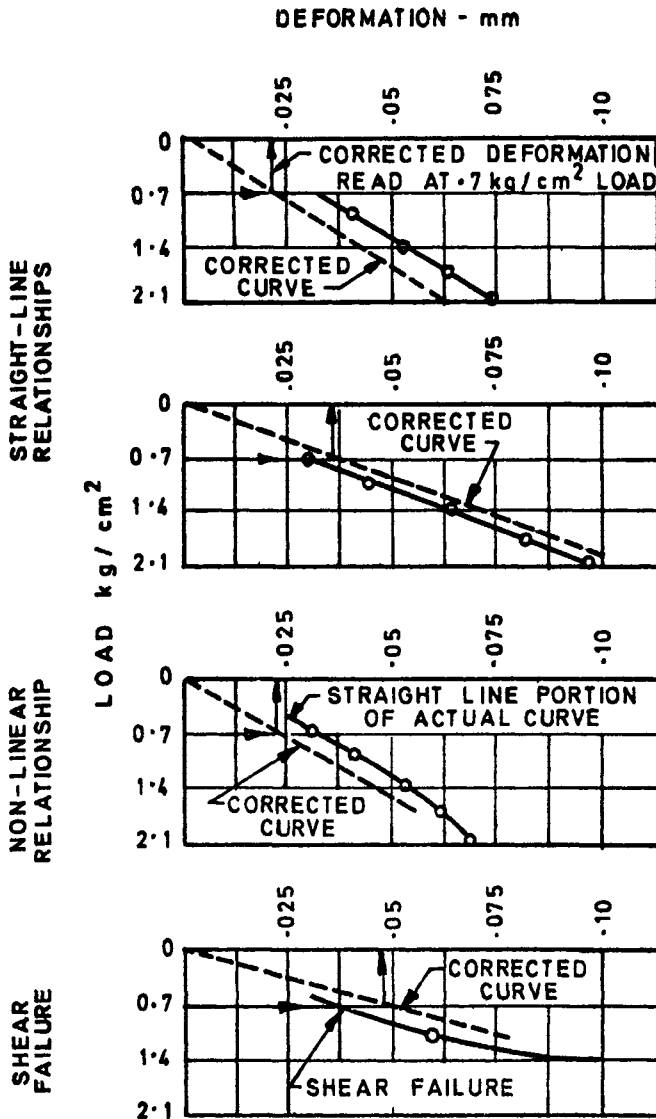
FIG. 4 CORRECTION OF LOAD-DEFLECTION CURVE
