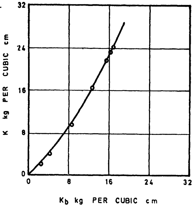
FIG. 5 CHART FOR CORRECTION FOR K_u FOR BENDING OF THE PLATE
