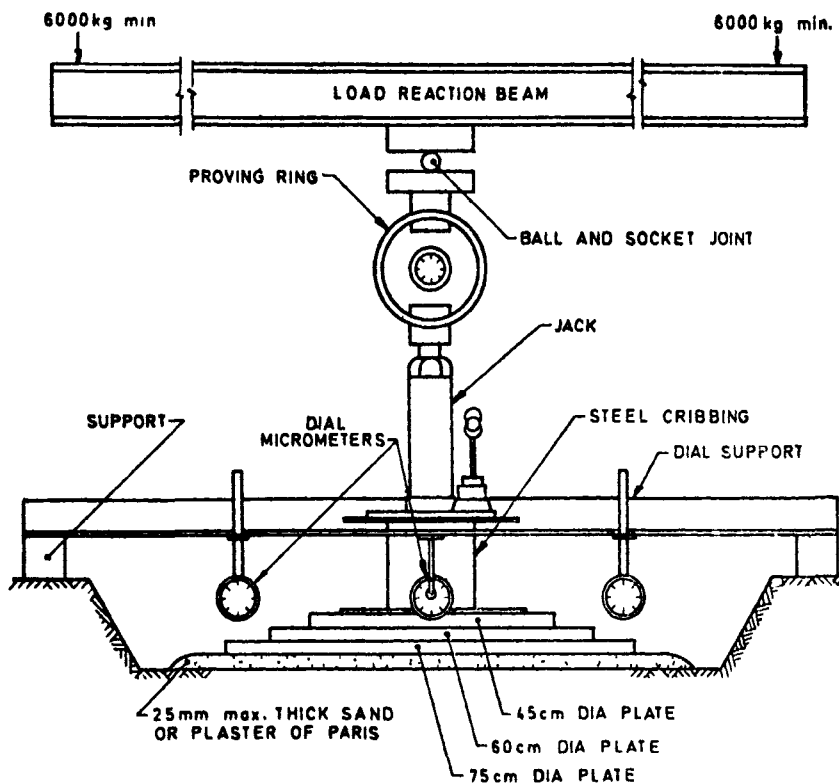
FIG. 2 SCHEMATIC DIAGRAM OF PLATE BEARING TEST
